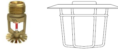
SPRINKLER + GUARD & WATER SHIELD ASSEMBLY
